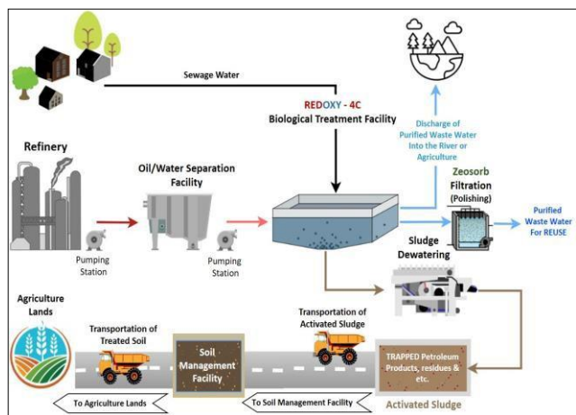
Treatment of Waste Water from the Refinery and Petrochemical Industry
